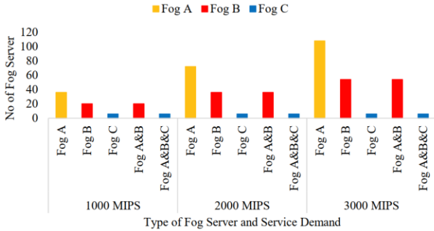
Fig. 6. Number of processing servers utilized in the fog-based approach with increasing traffic for different processing server capacities.
