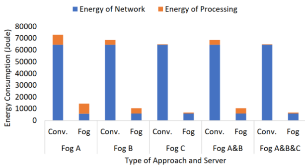
Fig. 3. Total energy consumption of fog-based approach and conventional approach for different processing server capacities.
