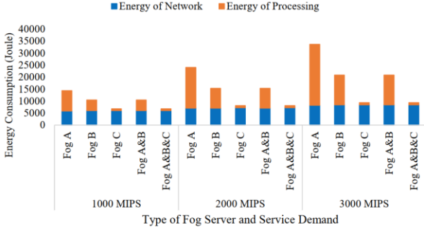
Fig. 5. Total energy consumption of the fog-based approach with increasing traffic for different processing server capacities.
