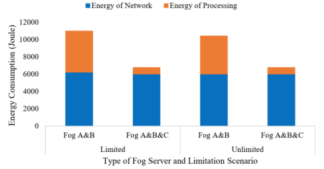
Fig. 7. Total energy consumption of the fog-based approach under limited and unlimited scenarios with different heterogeneous combinations of processing servers.
