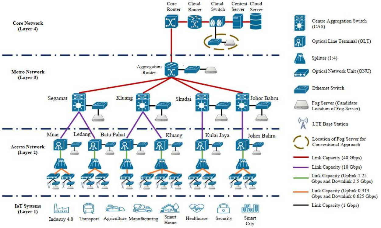
Fig. 1. Proposed Fog Computing Architecture.
