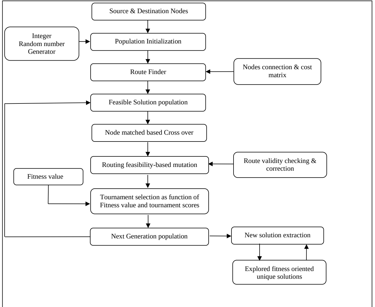
Fig. 1. Flowchart of the modified genetic algorithm for fitness-oriented routing optimization.
