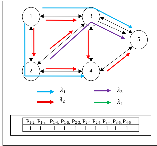
Fig. 5. Wavelength assignment with fittest routing (different colors indicates different wavelength).
