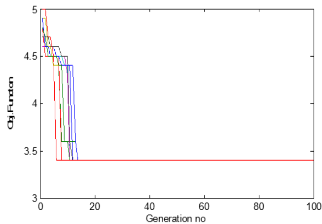
Fig. 4. Convergence characteristics over 10 trials with four routing options.
