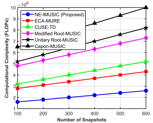
Fig. 5. Average CPU time versus number of snapshots for different DOA estimation algorithms.
