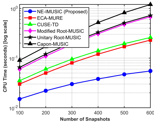
Fig. 6. CPU time growth comparison under increasing snapshot conditions.
