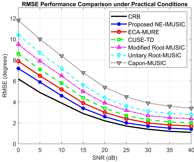
Fig. 8. RMSE versus SNR comparison of the proposed NE-IMUSIC algorithm with existing DOA estimation methods for a ULA with M = 12 sensors and P = 5 sources.
