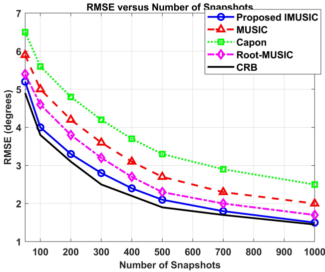
Fig. 9. RMSE versus number of snapshots comparison for different DOA estimation algorithms with M = 12 sensors and P = 5 sources.
