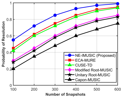
Fig. 4. Probability of resolution versus number of snapshots.
