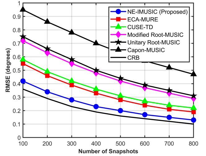
Fig. 2. RMSE vs number of snapshots.
