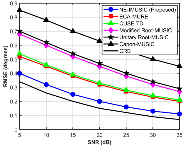
Fig. 1. RMSE vs SNR for various DOA estimation algorithms.
