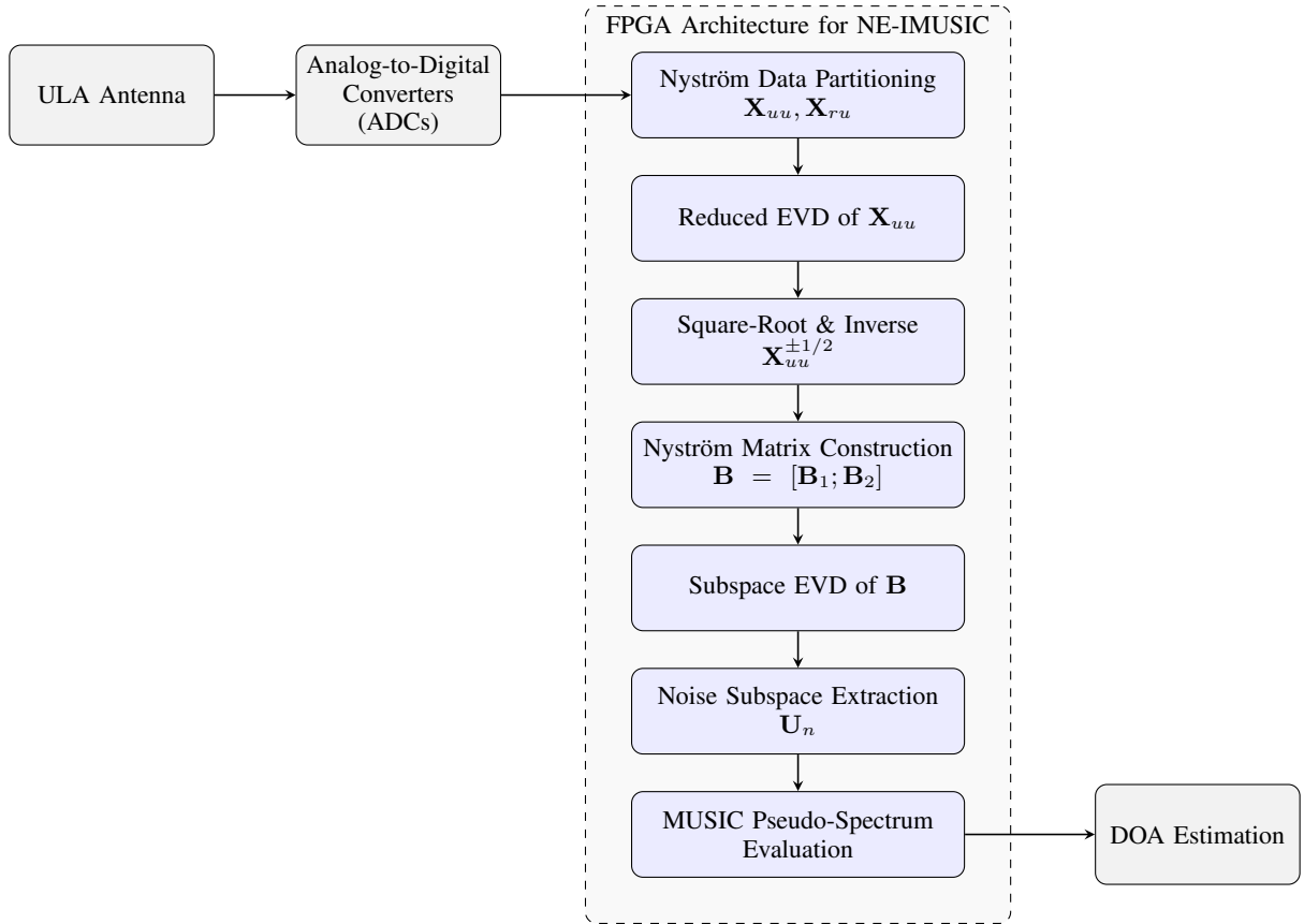
Fig. 7. FPGA architecture of the proposed NE-IMUSIC method.
