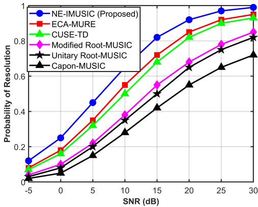
Fig. 3. Probability of resolution versus SNR.
