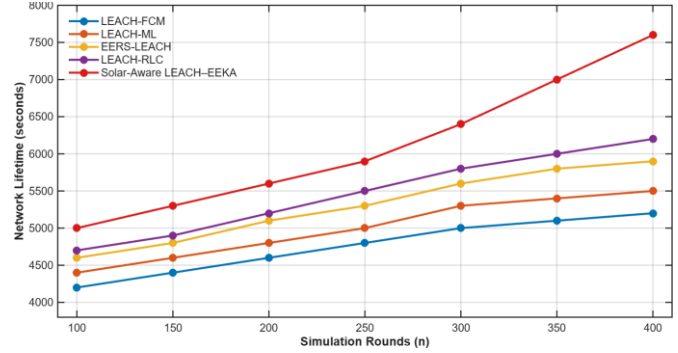
Fig. 4. Network Lifetime Comparison.
