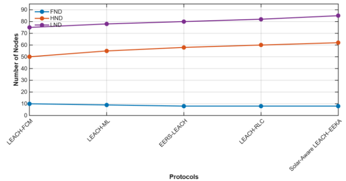
Fig. 9. Network Lifetime (FND, HND, and LND)
