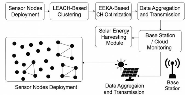
Fig. 2. The Architecture of Solar-Aware LEACH-EEKA.
