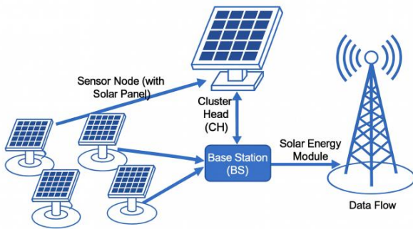
Fig. 1. Basic Structure of WSNs.
