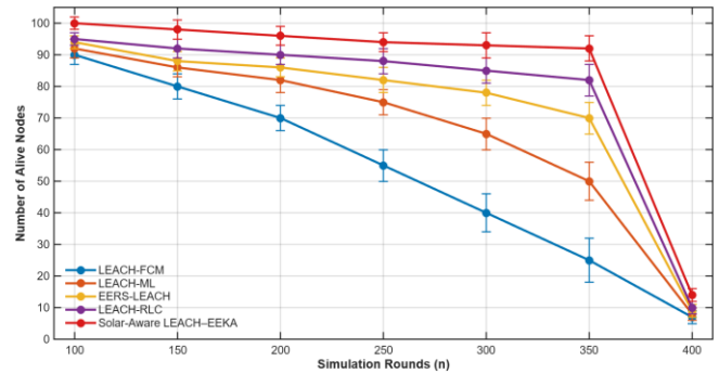
Fig. 8. Alive Nodes Comparison.
