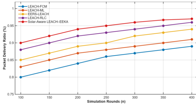
Fig. 7. PDR Comparison.
