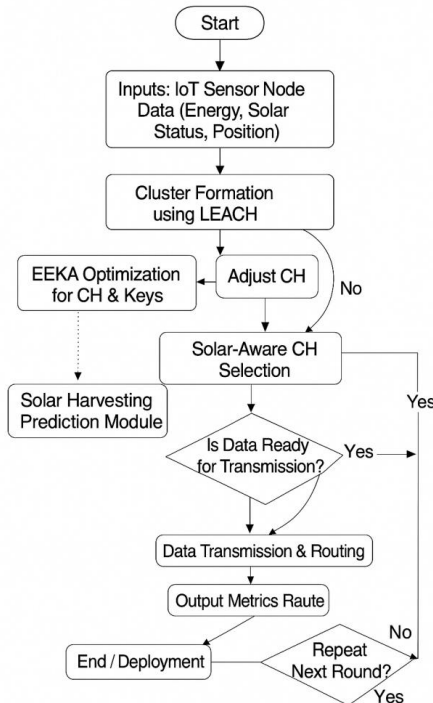
Fig. 3. Flow chart of Solar-Aware LEACH-EEKA.
