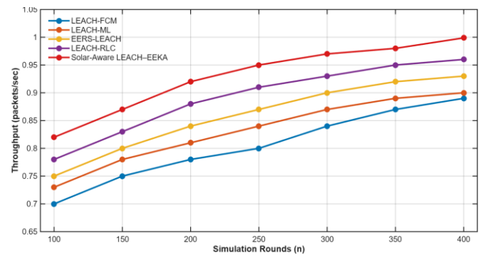
Fig. 6. Throughput Comparison.
