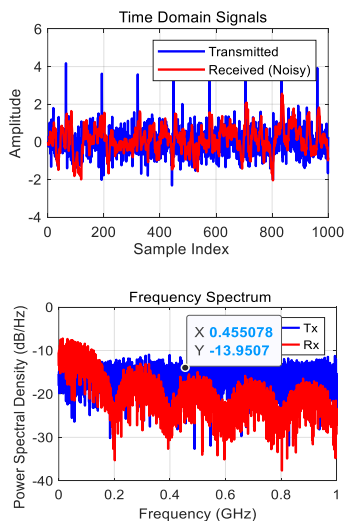
Fig. 1. Case 24 GHz simulation results.
