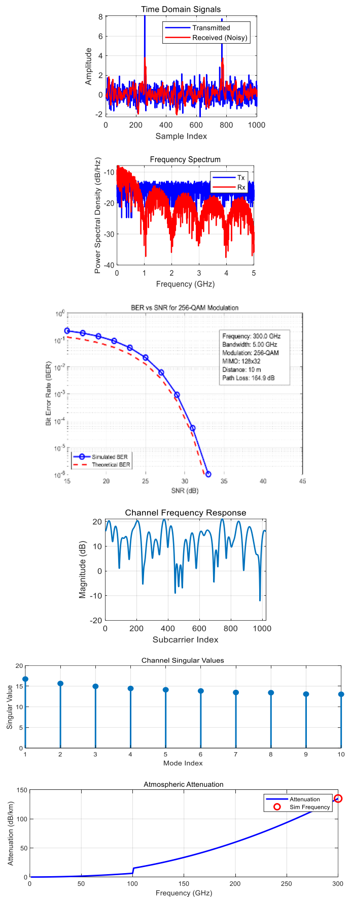
Fig. 4. Case 300 GHz simulation results.
