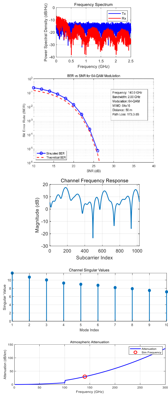
Fig. 3. Case 140 GHz simulation results.
