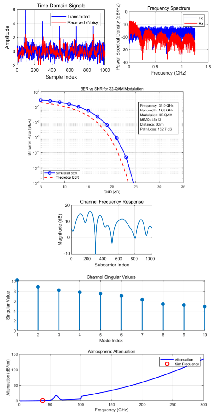
Fig. 6. Case 38 GHz simulation results.
