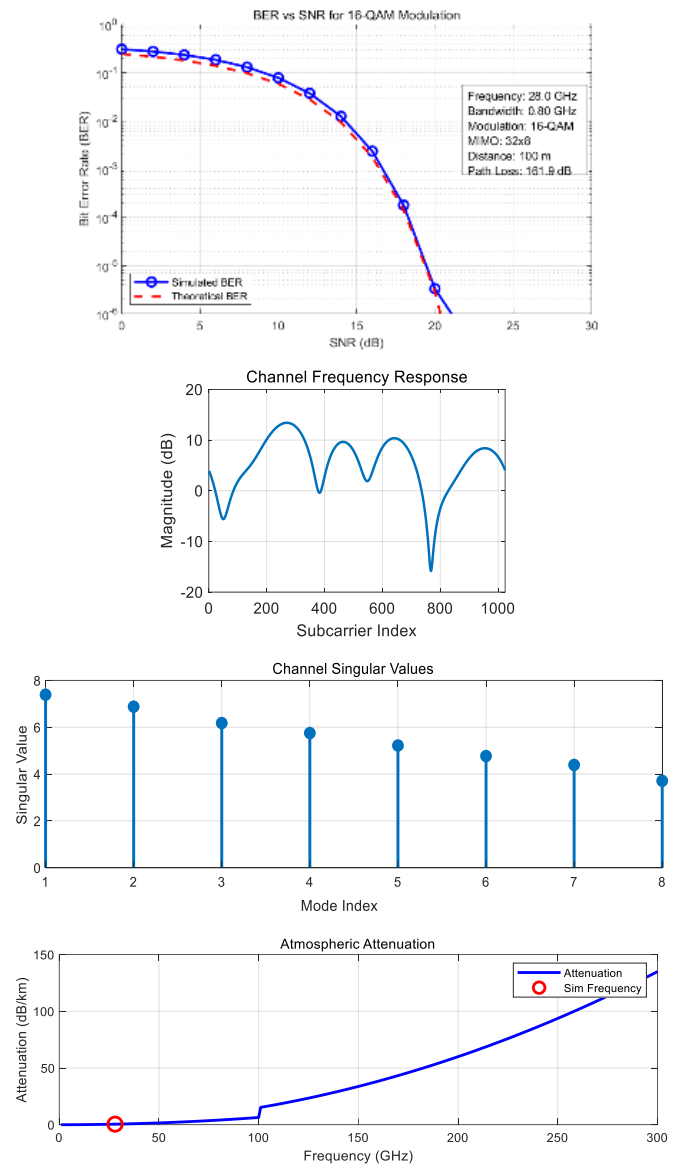
Fig. 2. Case 28 GHz simulation results.
