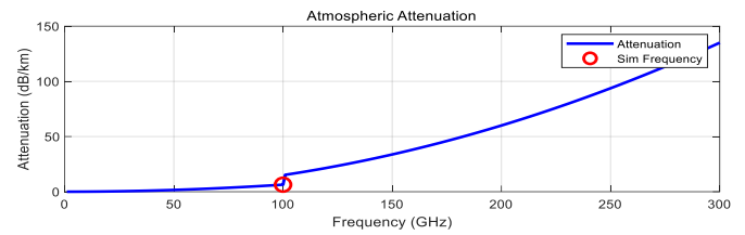
Fig. 5. Case 100 GHz simulation results
