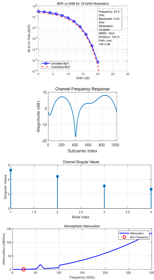
Fig. 1. Case 24 GHz simulation results.
