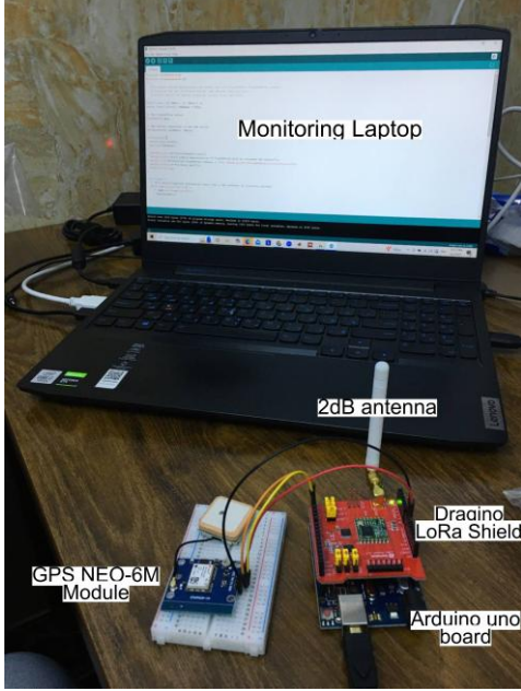
Fig. 5. Experimental testbeds.
