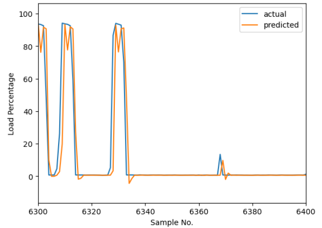
Fig. 5. Test performance of LSTM Model.
