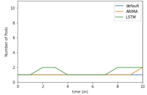
Fig. 9. Average active pods of various models.
