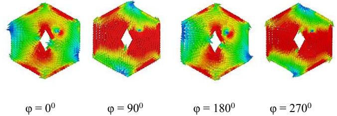
Fig. 6. Surface current distribution of LHCP antenna
