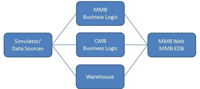
Fig. 2. Component architecture
