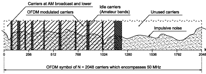
Fig. 1. The IEEE 1901 broadcast tone mask for North America mixed with a typical impulsive noise distribution in the frequency domain
