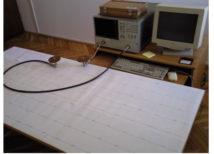
Fig. 4. Measurement setup
