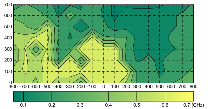
Fig. 11. Estimated coherence bandwidth at correlation threshold C_2
