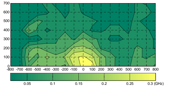
Fig. 10. Estimated coherence bandwidth at correlation threshold C_1
