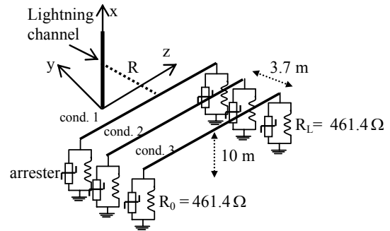
Fig. 2. Geometry considered.
